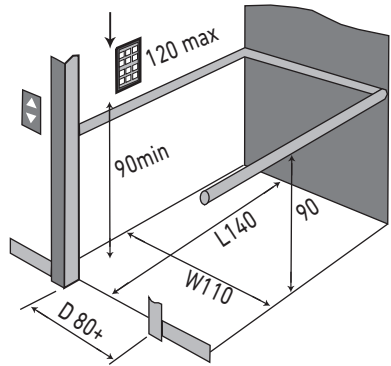
Passenger lift (with sliding doors)
