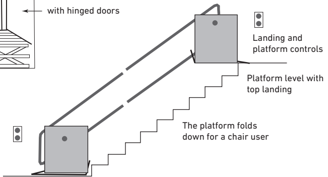
Wheelchair/platform stairlift
